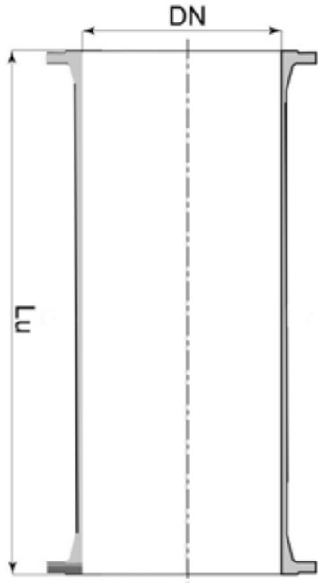
Niple Brida-Brida
